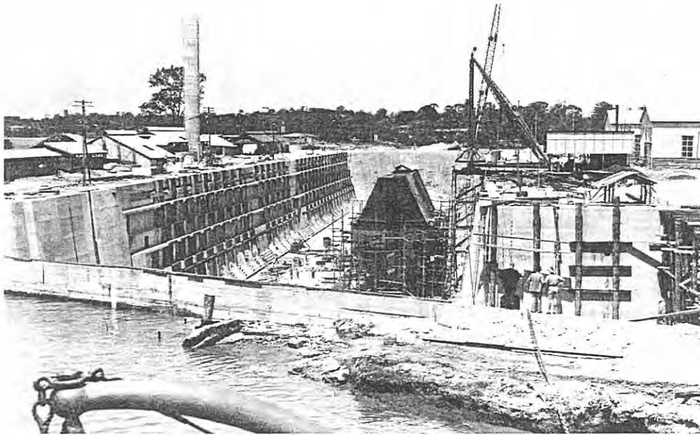
Cairncross Dock under construction, 14 February, 1944.
